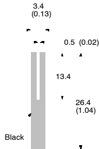
0.5-mm (0.02) wide Seal Slit (Two slits are provided)
