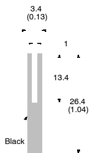
1-mm (0.04) wide Seal Slit (Two slits are provided)
