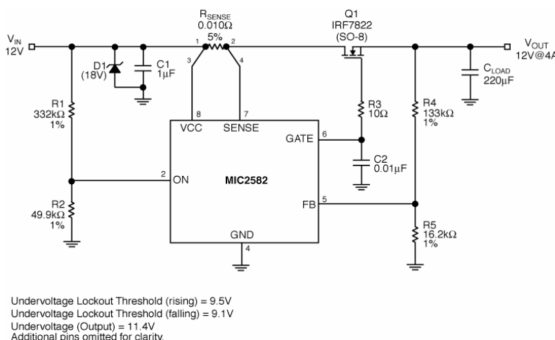
Figure 7. Higher UVLO Settings
