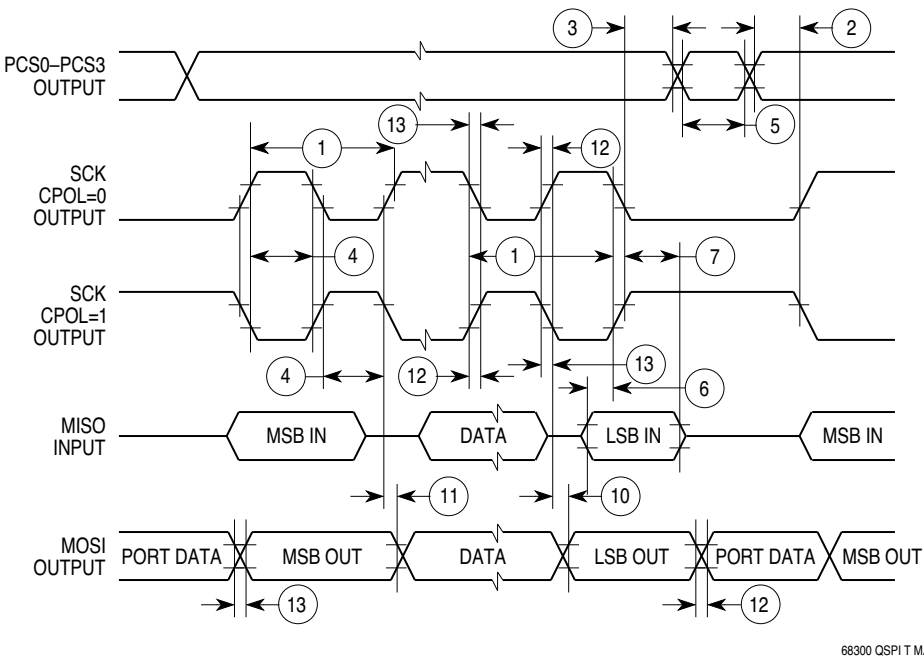
Figure A-17 QSPI Timing — Master, CPHA = 1
