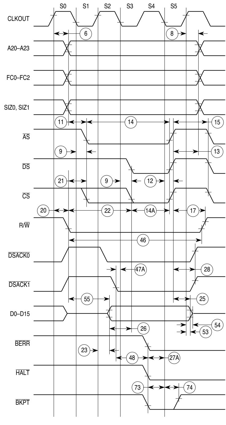
Figure A-4 Read Cycle Timing Diagram
