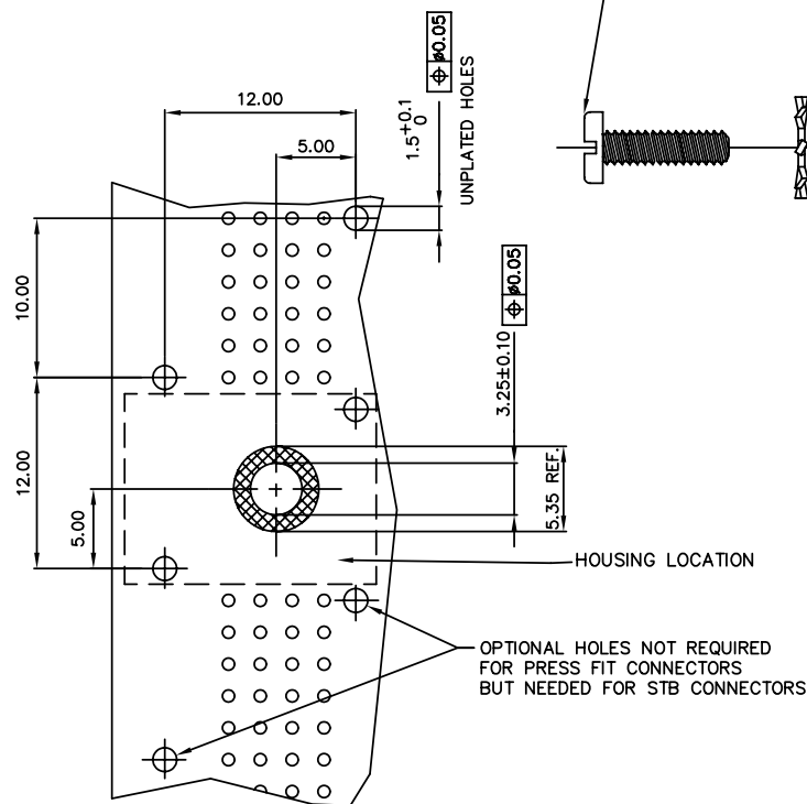
POWER PIN ASSEMBLY STYLE A
