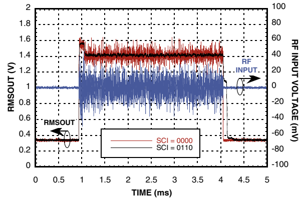
Residual Ripple for 2.6 GHz WiBro @ SCI = 0110
