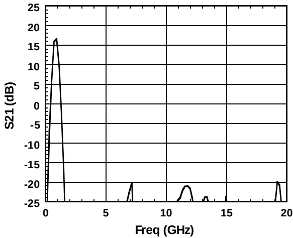
NJG1106KB2 S21 vs. Freq(to 20GHz)
