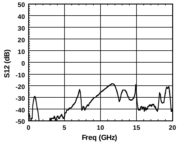
NJG1106KB2 S12 vs. Freq(to 20GHz)
