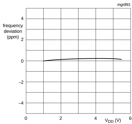
Fig 27. Frequency deviation as a function of supply voltage V_{DD}
