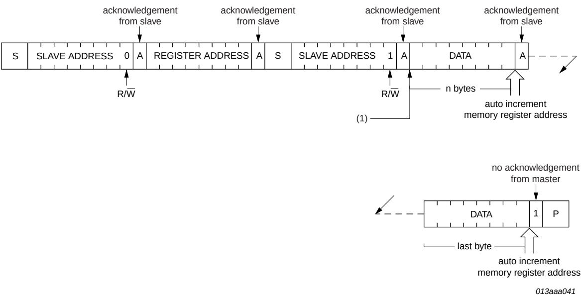
Fig 20. Master reads after setting register address (write register address; READ data)
