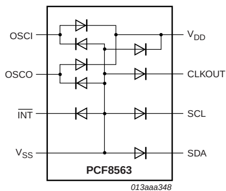
Fig 23. Device diode protection diagram
