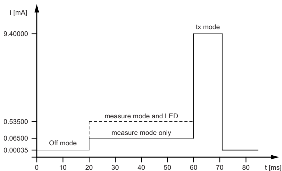
Figure 3-3. Remote Sensor Current Consumption at 24°C
