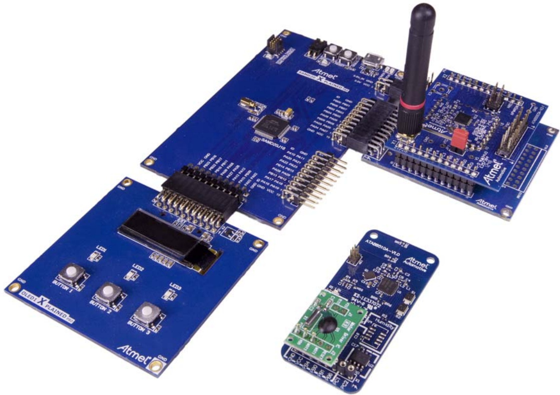
Figure 1-2. ATA8510-EK1 Kit
