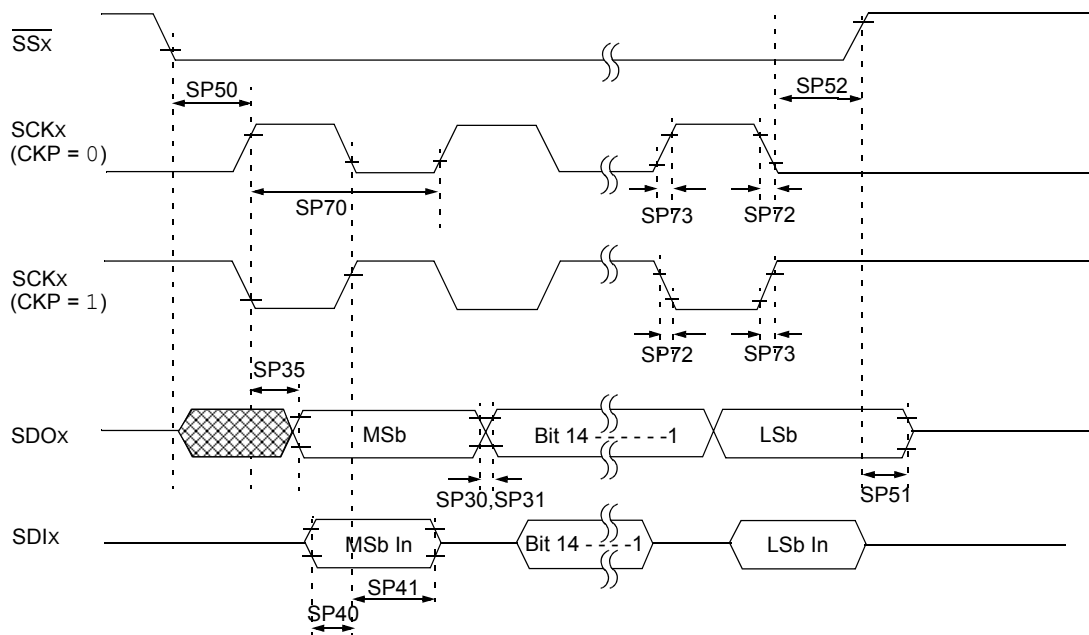
FIGURE 22-15: SPIx SLAVE MODE (FULL-DUPLEX CKE = 0, CKP = 1, SMP = 0) TIMING CHARACTERISTICS
