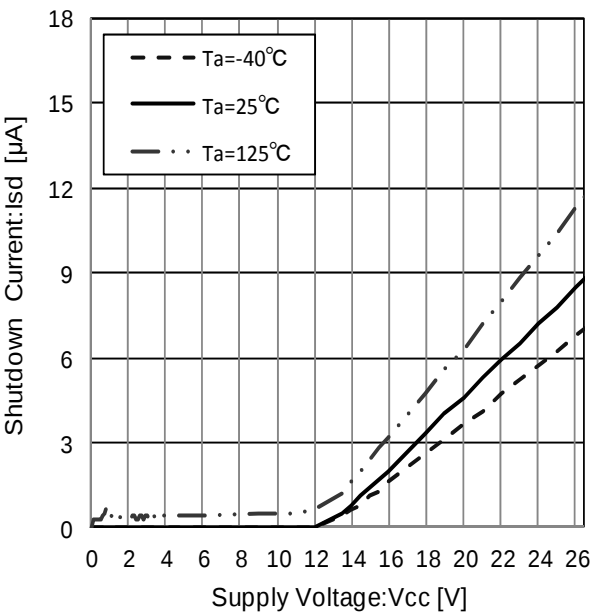
Figure 24. Shutdown Current
