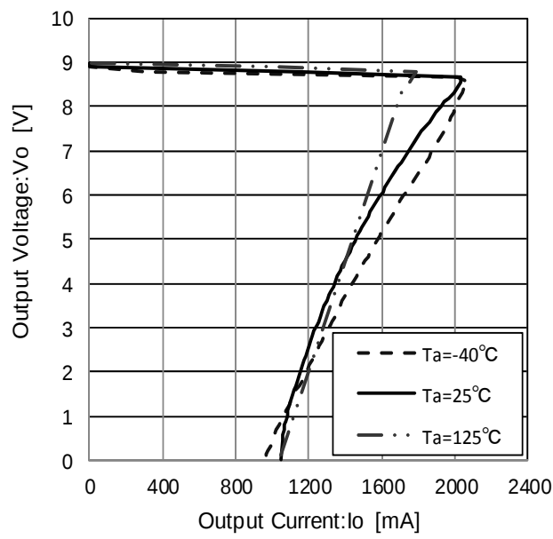
Figure 62. Load Regulation
