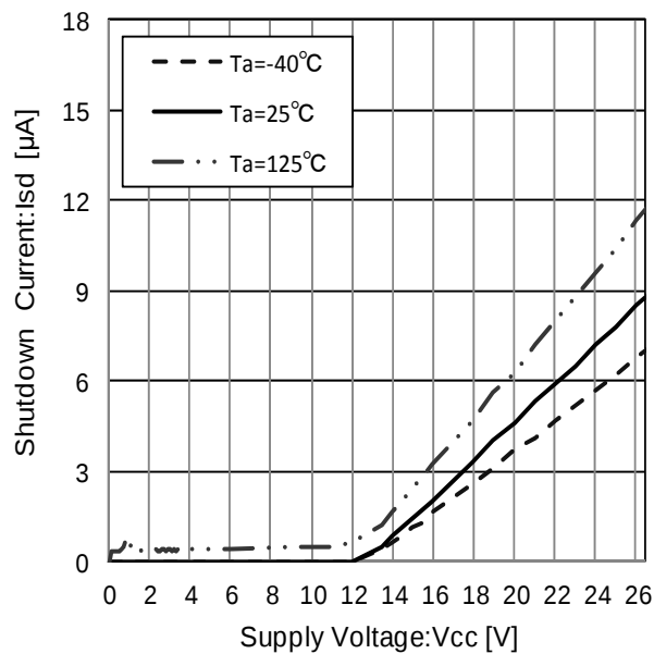
Figure 35. Shutdown Current
