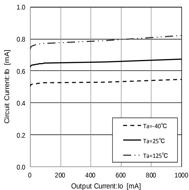
Figure 30. Circuit Current
