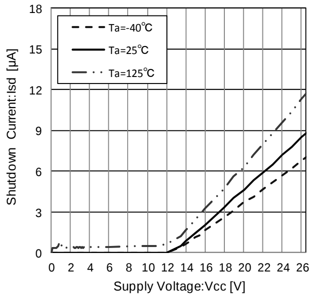
Figure 12. Shutdown Current
