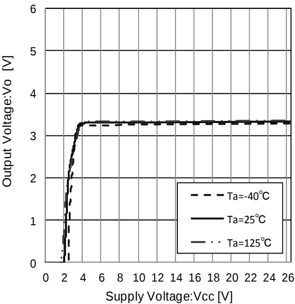
Figure 26. Line Regulation ( I_o=500\text{mA} )
