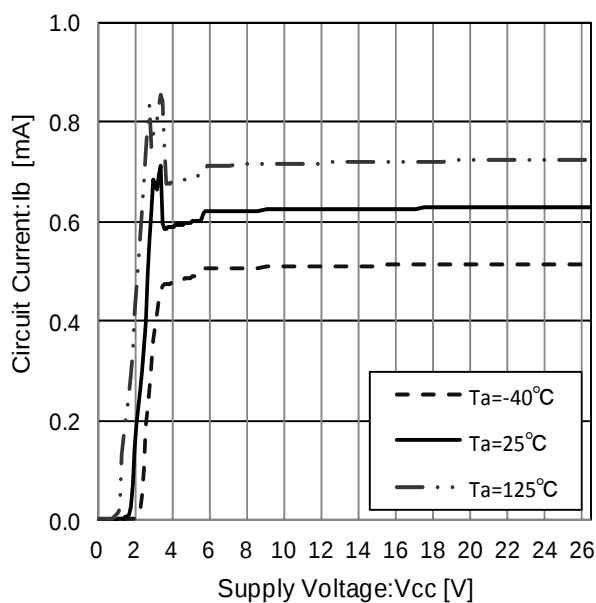
Figure 23. Circuit Current
