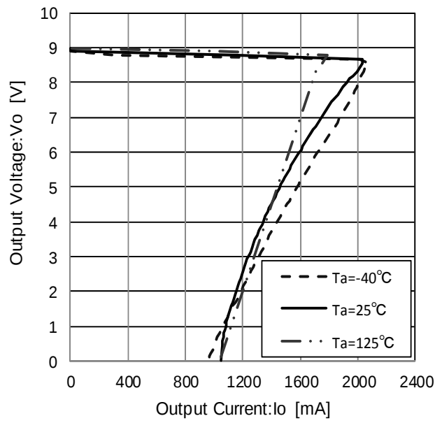
Figure 62. Load Regulation
