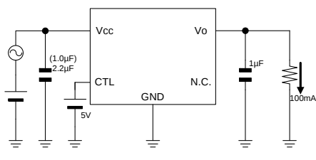
Measurement setup for Figure 28, 40, 52 and 64
