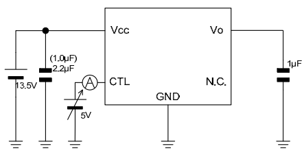
Measurement setup for Figure 31, 43, 55 and 67
