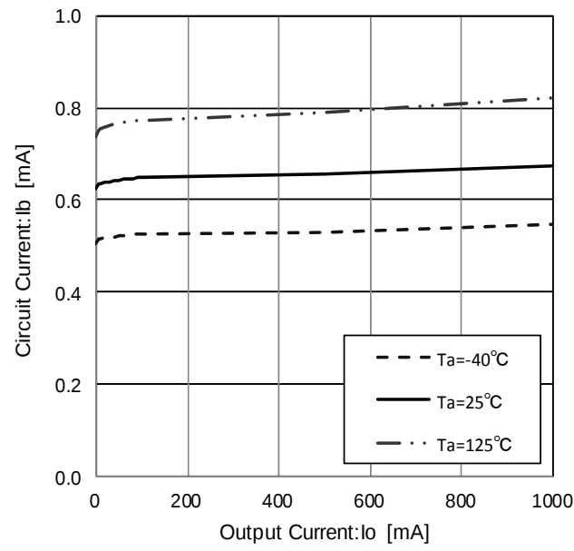
Figure 42. Circuit Current
