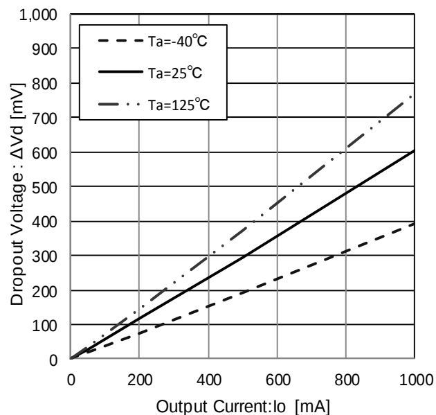
Figure 16. Dropout Voltage (V CC =V O ×0.95, 0mA ≤ I O ≤ 1000mA)
