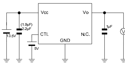
Measurement setup for Figure 33, 45, 57 and 69
