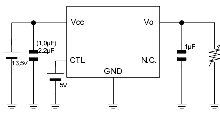
Measurement setup for Figure 30, 42, 54 and 66
