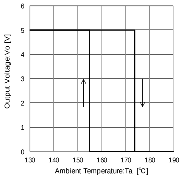
Figure 45. Thermal Shutdown Circuit Characteristic
