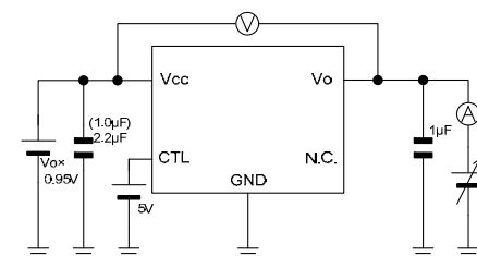
Measurement setup for Figure 39, 51 and 63
