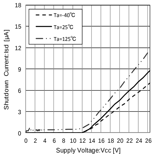
Figure 24. Shutdown Current
