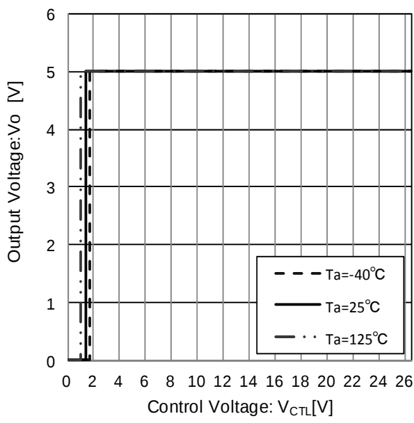
Figure 21. CTL Voltage vs Output Voltage
