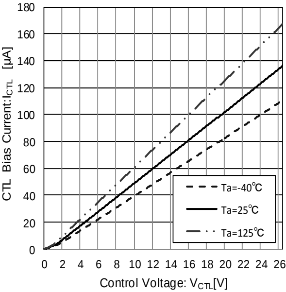
Figure 67. CTL Voltage vs CTL Current
