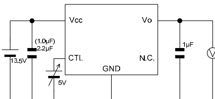
Measurement setup for Figure 32, 44, 56 and 68
