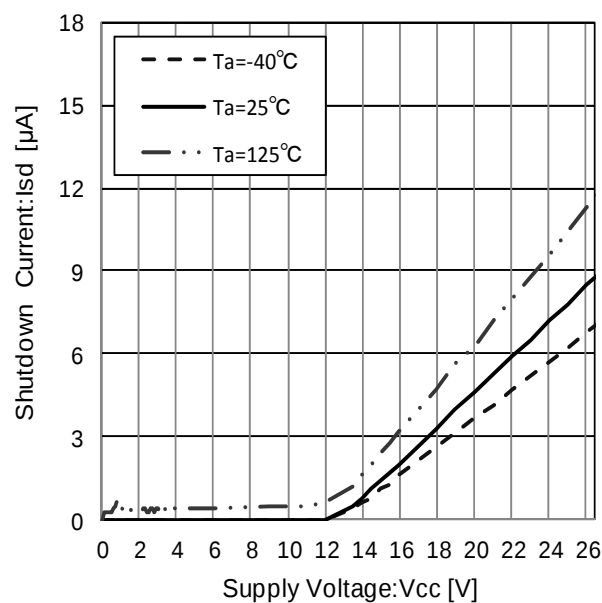
Figure 47. Shutdown Current
