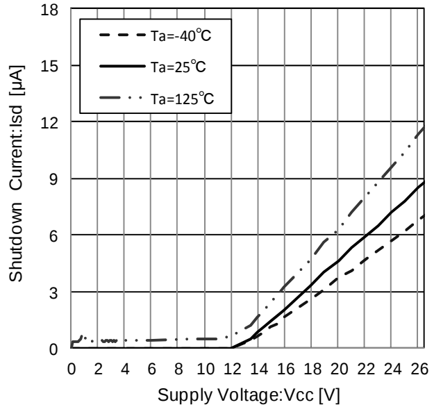
Figure 12. Shutdown Current
