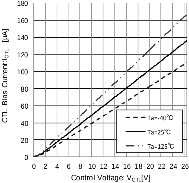
Figure 55. CTL Voltage vs CTL Current
