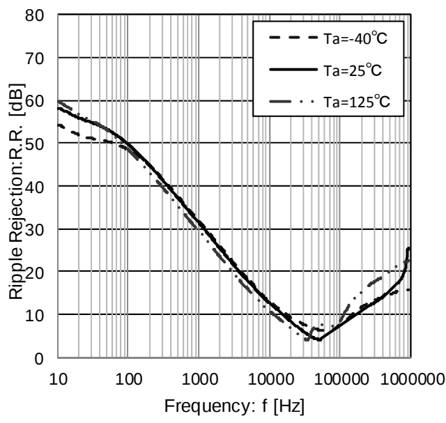
Figure 64. Ripple Rejection ( I_o = 100\text{mA} )
