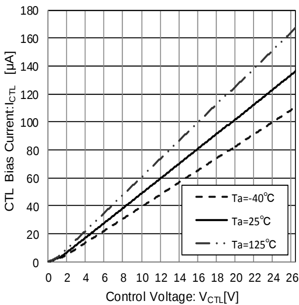
Figure 43. CTL Voltage vs CTL Current
