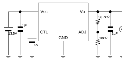
Measurement setup for Figure 22
