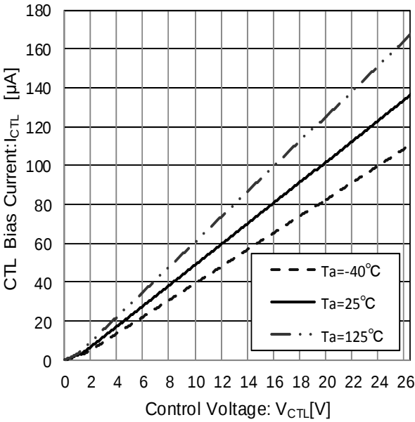
Figure 67. CTL Voltage vs CTL Current
