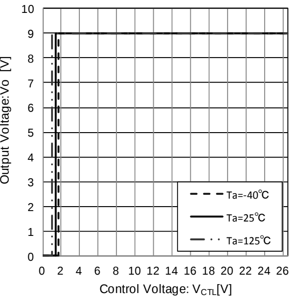
Figure 68. CTL Voltage vs Output Voltage
