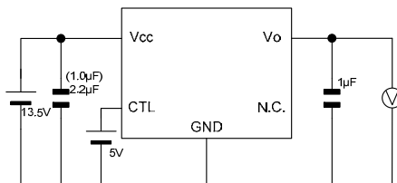
Measurement setup for Figure 33, 45, 57 and 69
