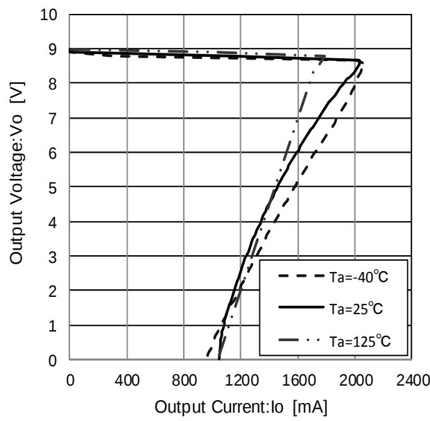
Figure 62. Load Regulation
