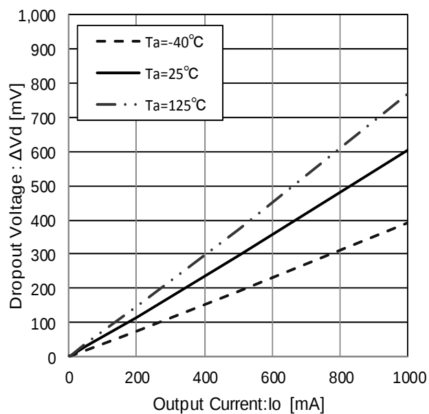
Figure 51. Dropout Voltage ( V_{CC}=V_O \times 0.95V )
