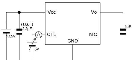
Measurement setup for Figure 31, 43, 55 and 67
