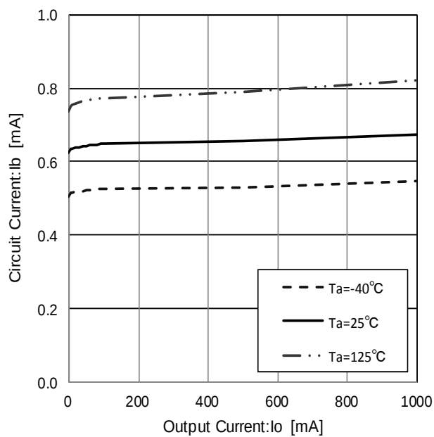
Figure 30. Circuit Current
