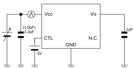
Measurement setup for Figure 23, 34, 46 and 58
