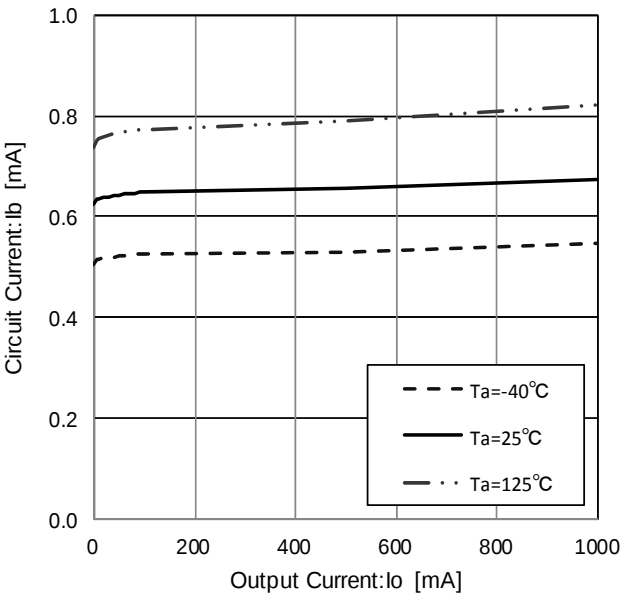
Figure 54. Circuit Current
