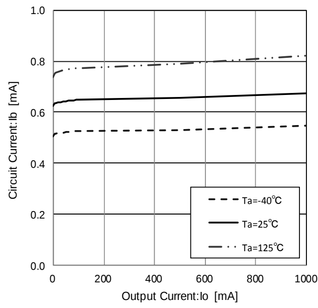
Figure 42. Circuit Current
