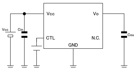
Figure 2. Typical Application Circuit Output Voltage Fixation Type (With Shutdown SW)
