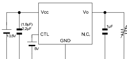
Measurement setup for Figure 30, 42, 54 and 66
