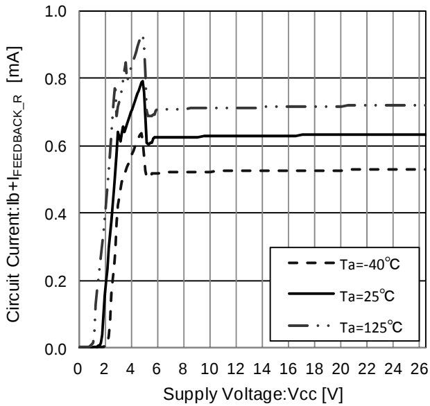
Figure 11. Circuit Current ( I_{FEEDBACK\_R} \approx 75\mu A )
