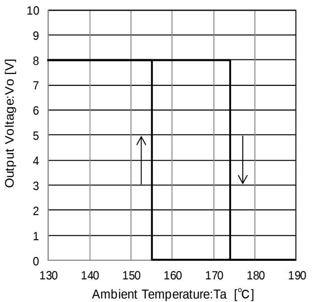
Figure 57. Thermal Shutdown Circuit Characteristic
