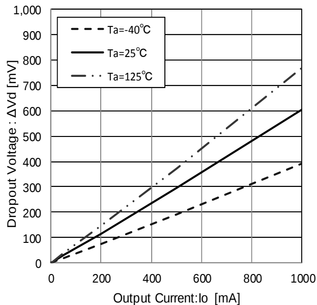
Figure 39. Dropout Voltage ( V_{cc} = V_o \times 0.95\text{V} )
