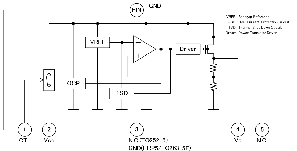
Figure 8. Block diagram BDxxC0AWFP/WHFP/WFP2-C (Output Voltage Fixation Type, with Shutdown SW)
