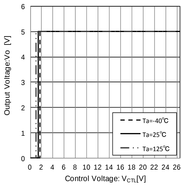
Figure 44. CTL Voltage vs Output Voltage
