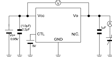
Measurement setup for Figure 39, 51 and 63
