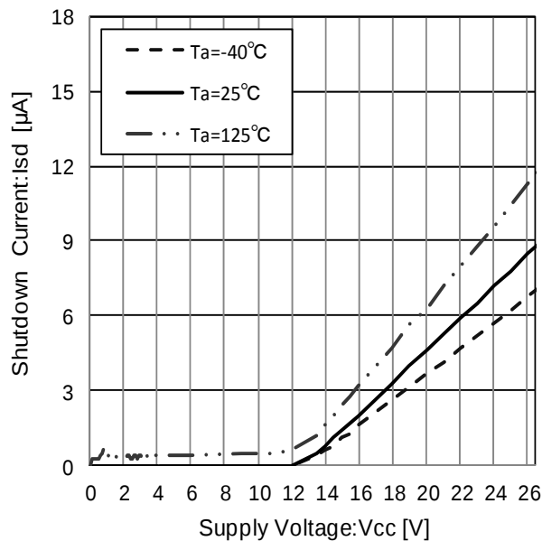
Figure 59. Shutdown Current
