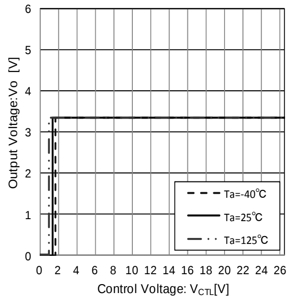
Figure 32. CTL Voltage vs Output Voltage
