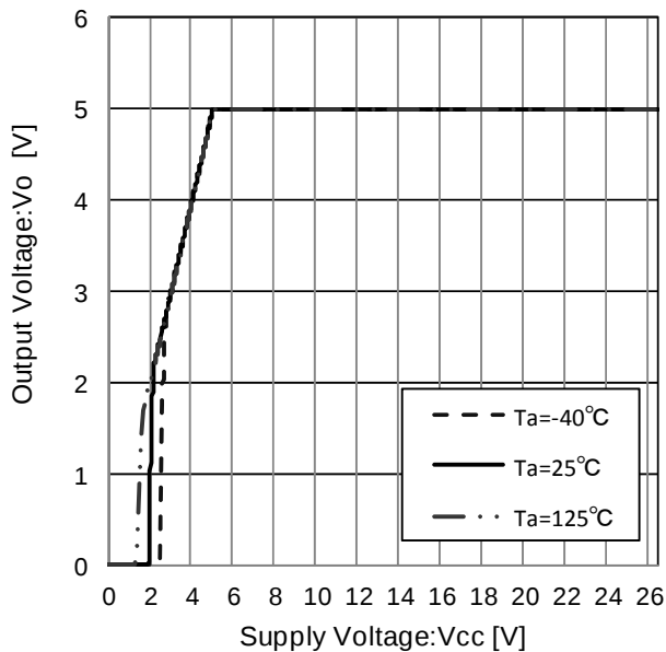
Figure 13. Line Regulation ( I_o=0mA )
