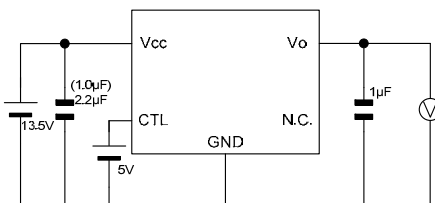
Measurement setup for Figure 29, 41, 53 and 65
