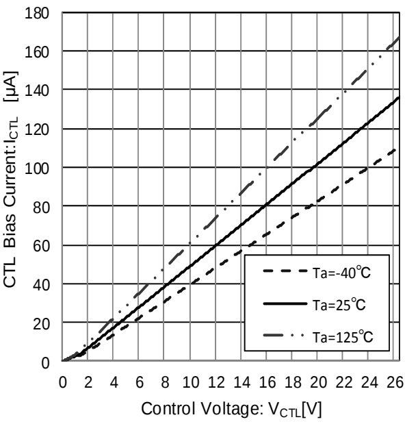
Figure 20. CTL Voltage vs CTL Current
