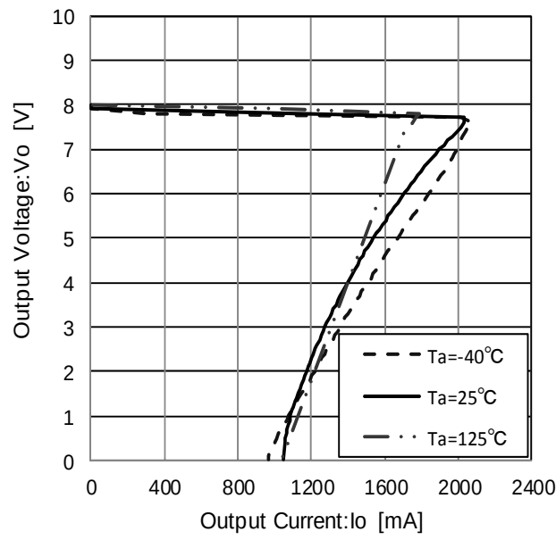
Figure 50. Load Regulation
