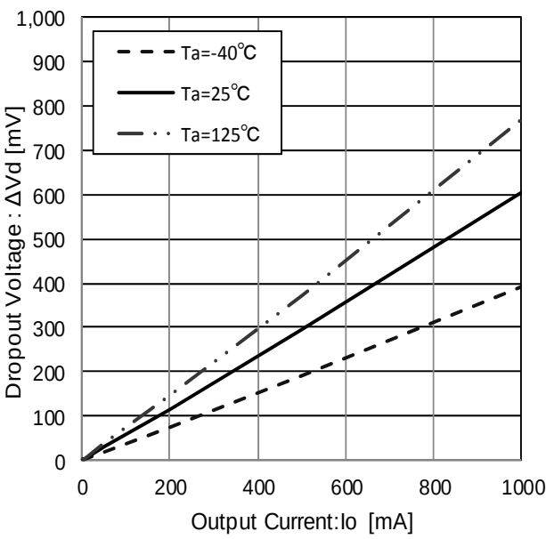
Figure 51. Dropout Voltage (Vcc=Vo×0.95V)
