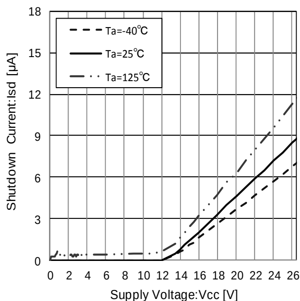
Figure 47. Shutdown Current
