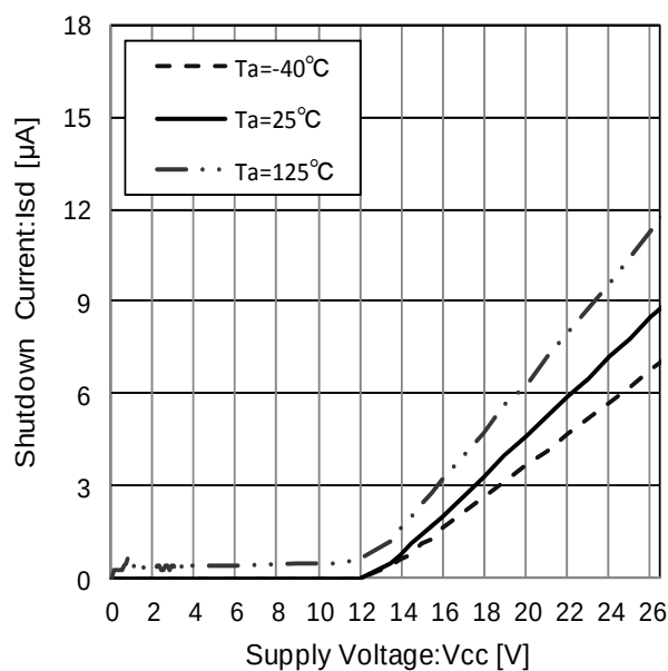
Figure 47. Shutdown Current
