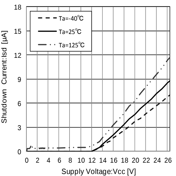
Figure 35. Shutdown Current
