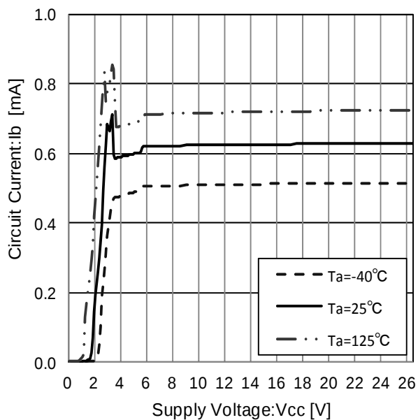
Figure 23. Circuit Current
