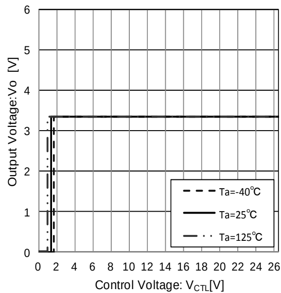
Figure 32. CTL Voltage vs Output Voltage
