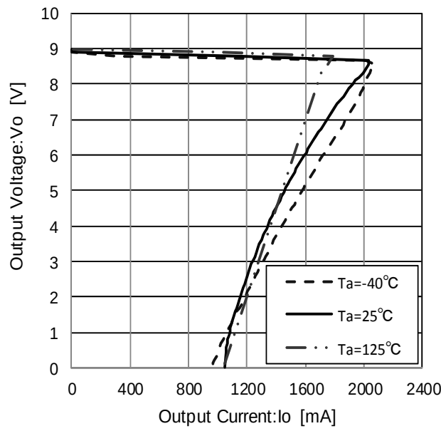
Figure 62. Load Regulation
