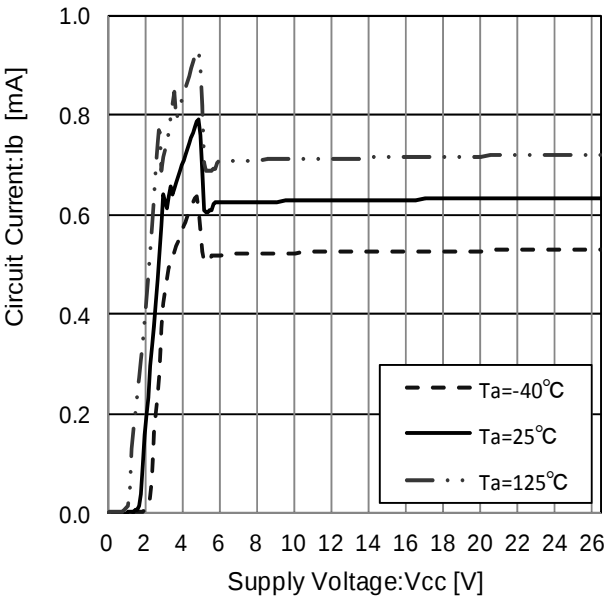
Figure 34. Circuit Current
