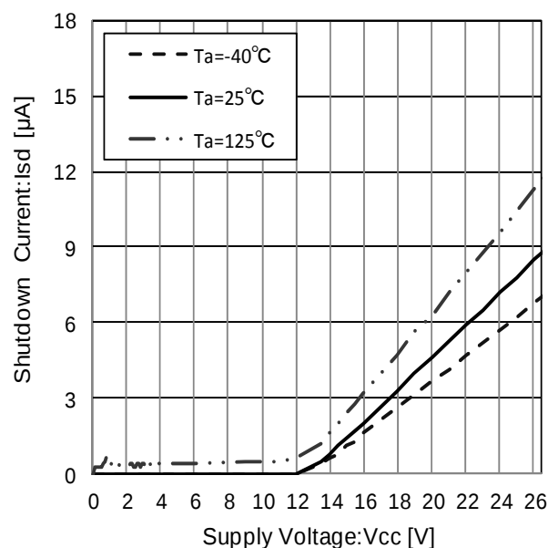
Figure 47. Shutdown Current
