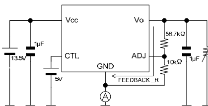
Measurement setup for Figure 19
