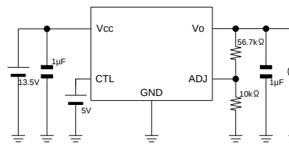
Measurement setup for Figure 22
