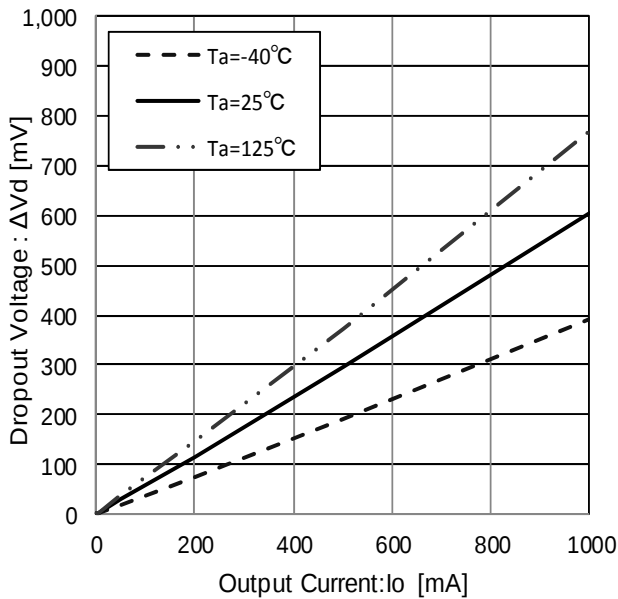
Figure 39. Dropout Voltage (V CC =V O ×0.95V)
