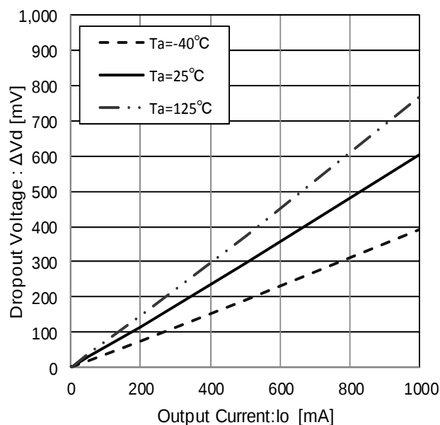
Figure 51. Dropout Voltage (V CC =V O ×0.95V)
