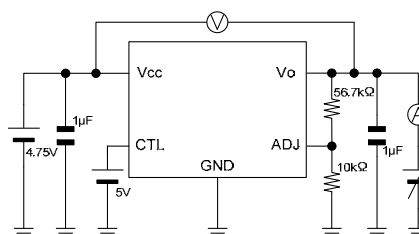
Measurement setup for Figure 16
