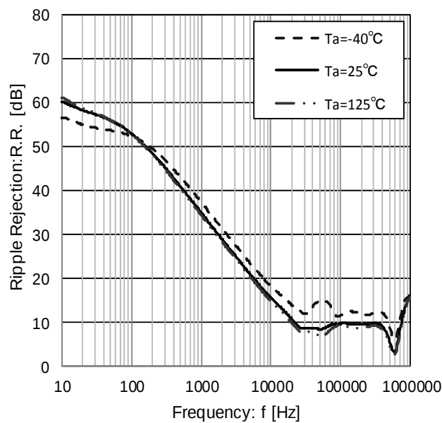
Figure 40. Ripple Rejection (I O =100mA)
