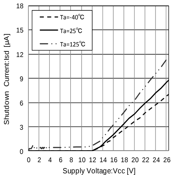
Figure 24. Shutdown Current
