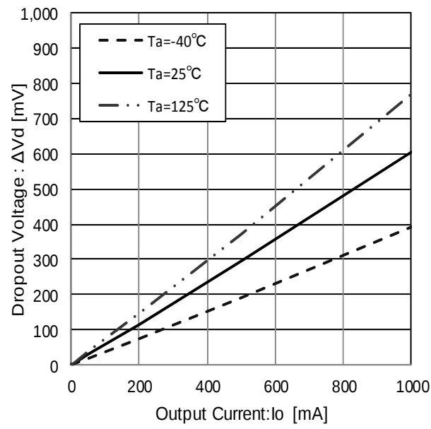
Figure 63. Dropout Voltage ( V_{cc} = V_o \times 0.95\text{V} )
