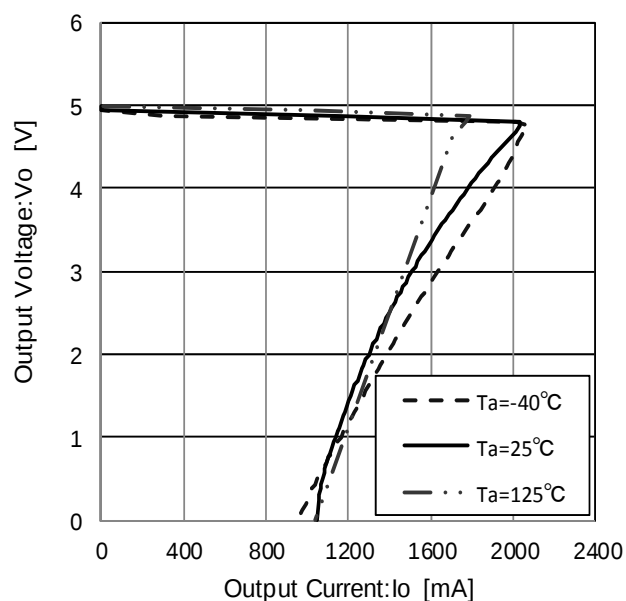
Figure 15. Load Regulation
