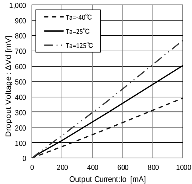
Figure 39. Dropout Voltage (V CC =V O ×0.95V)
