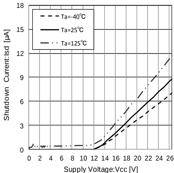
Figure 59. Shutdown Current
