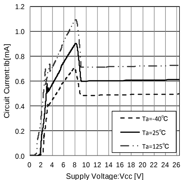
Figure 58. Circuit Current
