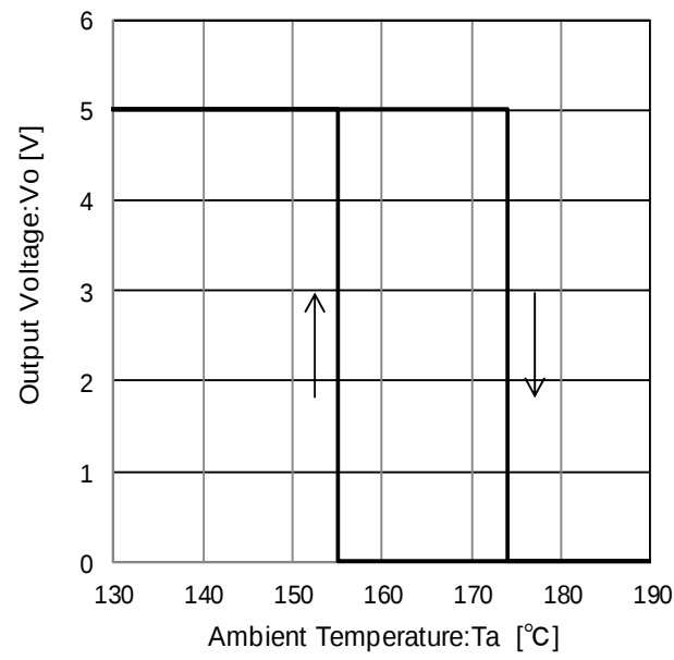
Figure 22. Thermal Shutdown Circuit Characteristic
