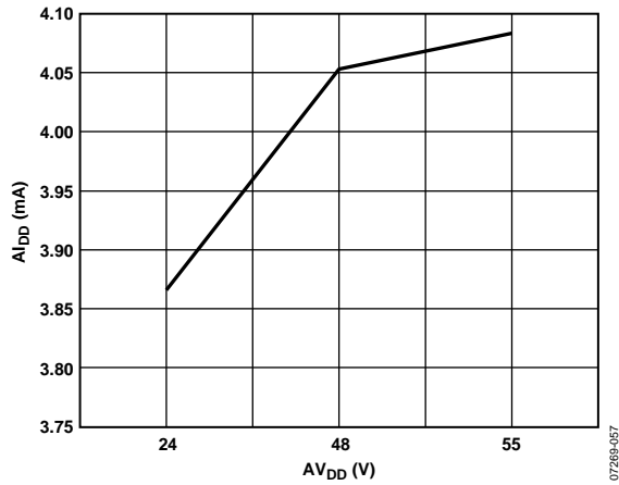
Figure 48. A_{I_{DD}} vs. AV_{DD} , V_{OUT} = 0\text{ V}
