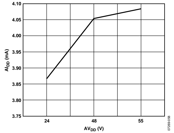
Figure 49. A_{I_{DD}} vs. AV_{DD} , I_{OUT} = 0\text{ mA}
