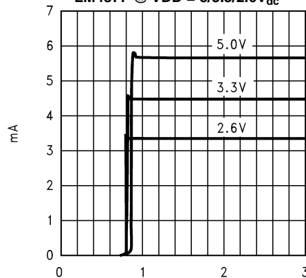
Volts – Pin 1 Figure 18.
