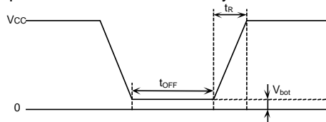
Figure 56. Rise Waveform Diagram
