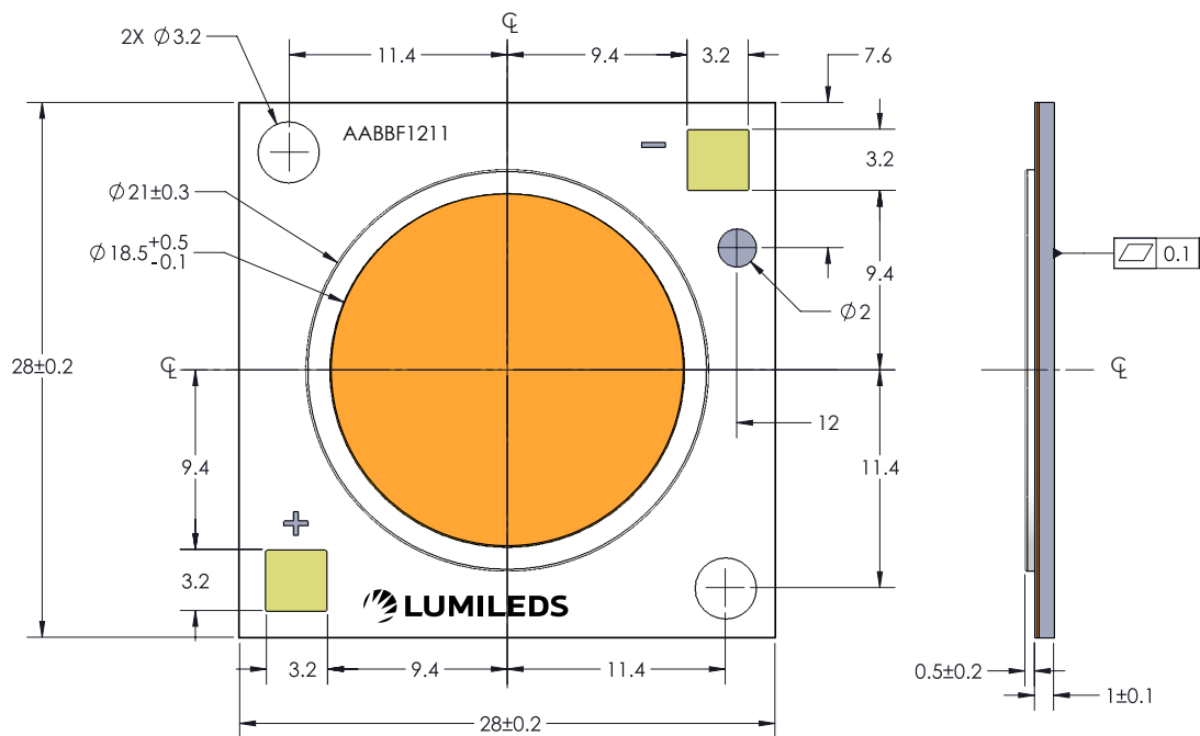
Figure 8g. Mechanical dimensions for L2C2-xxxx1211E1900.
