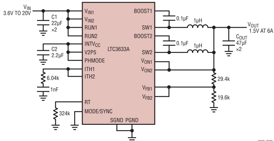
1.5V 1MHz Dual Phase Buck Regulator
