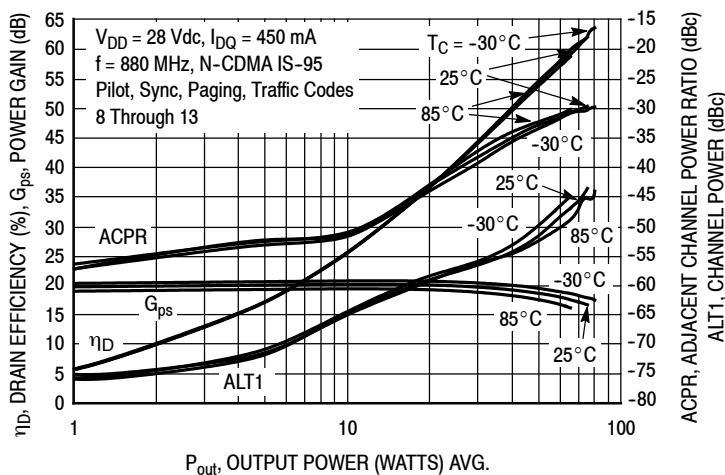
Figure 11. Single-Carrier N-CDMA ACPR, ALT1, Power Gain and Drain Efficiency versus Output Power
