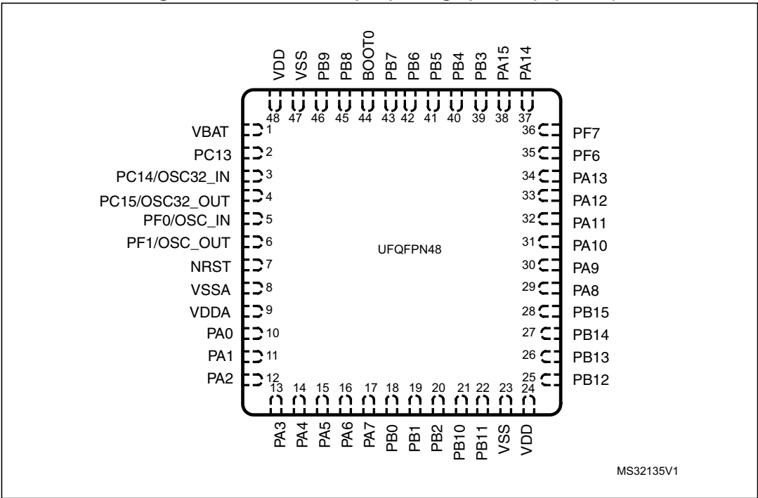
Figure 6. UFQFPN48 48-pin package pinout (top view)
