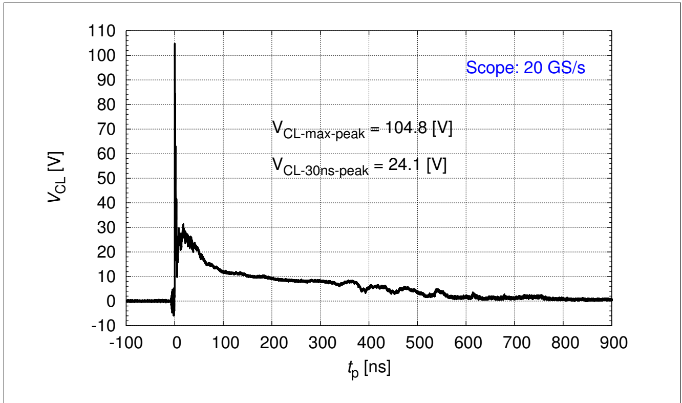
Figure 3-7 IEC61000-4-2: V_{CL} = f(t) , 15 kV positive pulse from pin 1 to pin 2 ( R = 330 \Omega , C = 150 pF)
