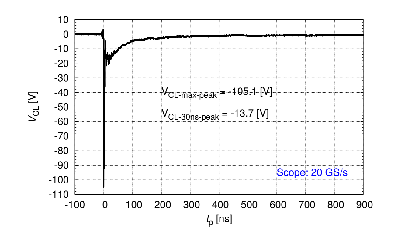
Figure 3-8 IEC61000-4-2: V_{CL} = f(t) , 15 kV negative pulse from pin 1 to pin 2 ( R = 330 \Omega , C = 150 pF)
