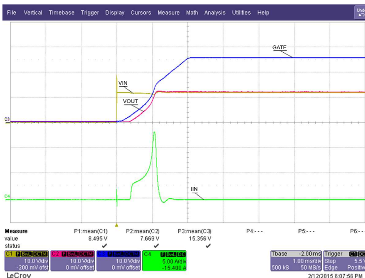
Figure 27. Startup
