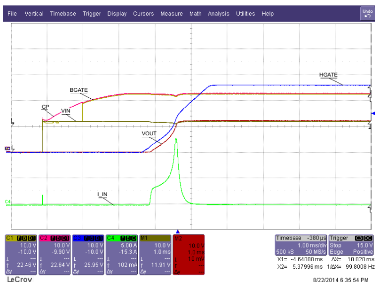
Figure 5. Startup ( C_O = 440 \mu\text{F} )
