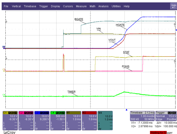
Figure 6. Startup ( C_O = 440 \mu\text{F} )
