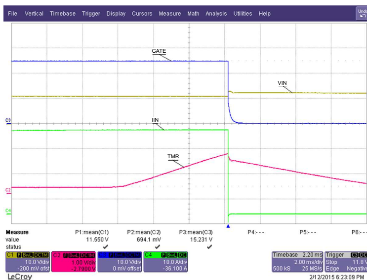
Figure 30. Overcurrent
