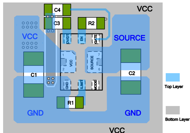
Figure 4: Recommended Layout
