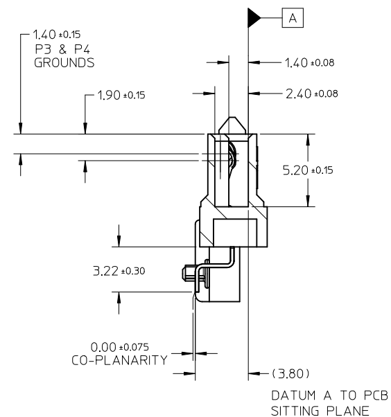
SECTION Z-Z
