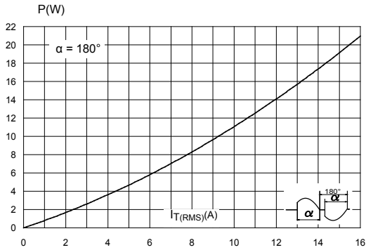
Figure 1. Maximum power dissipation versus on-state RMS current
