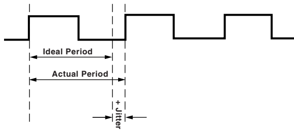
Figure 22: Period Tolerance and Clock Jitter
