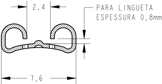
SECTION X-X SCALE 5:1
