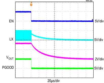
MAXM17624 SHUTDOWN THROUGH ENABLE ( V_{IN} = 5V , V_{OUT} = 3.3V , I_{LOAD} = 1A , PWM MODE)
