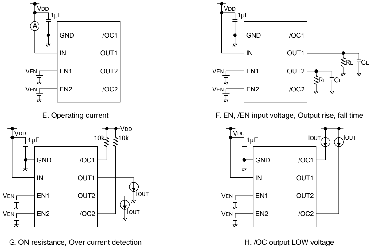
Figure 1. Measurement circuits
