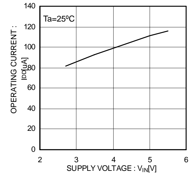
Figure 49. Operating current EN,/EN Enable
