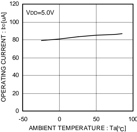
Figure 4. Operating current
