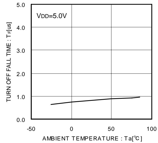
Figure 14. Output fall time
