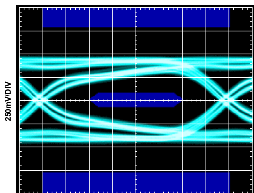
Figure 5. Rx Eye Diagram at TP2 (Cable = 2 Meters, 24 AWG)
