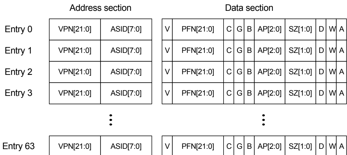
Figure 5-5. TLB organization
