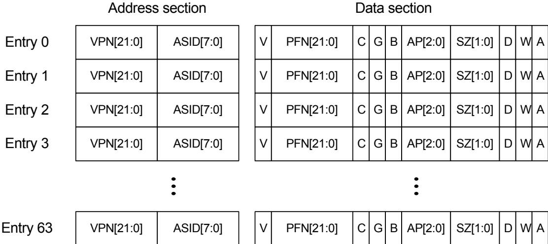
Figure 5-5. TLB organization
