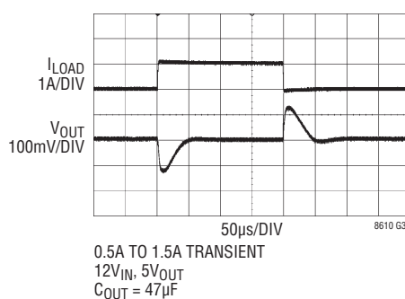
Transient Response
