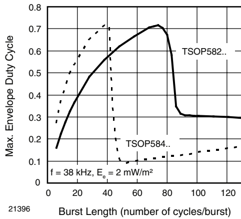
Fig. 9 - Max. Envelope Duty Cycle vs. Burst Length
