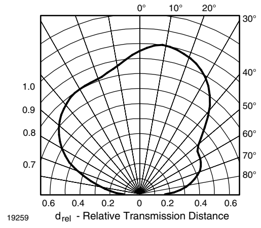
Fig. 13 - Vertical Directivity
