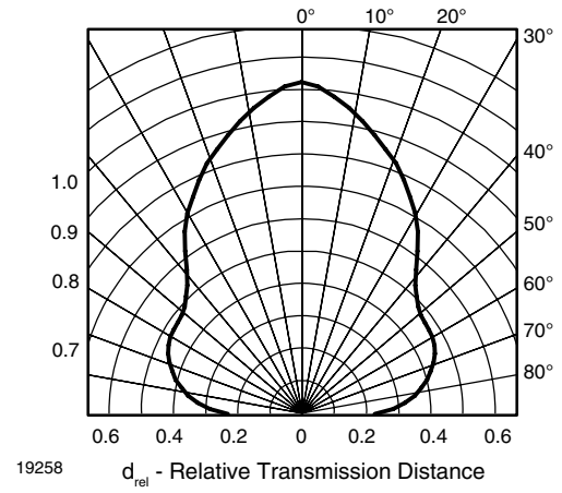
Fig. 12 - Horizontal Directivity
