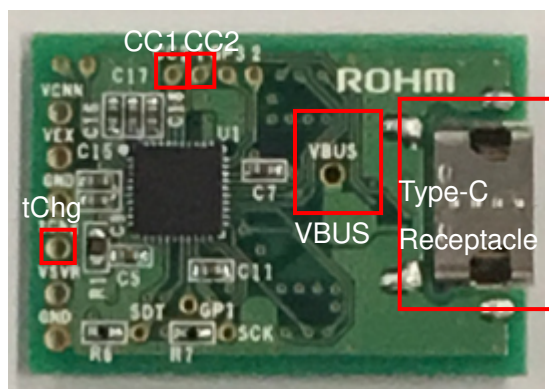
Figure3. Evaluation Board Photo
