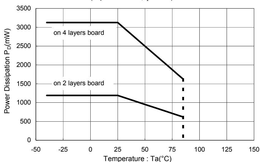
NJW4185DL3 PowerDissipation ( T_{opr} = -40 \sim +85^\circ C , T_j = 150^\circ C )
