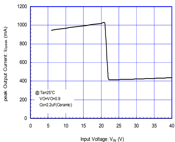
NJW4185_5.0V Peak Output Current vs. Input Voltage
