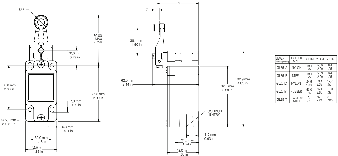
Figure 2. Fixed Lever, Side Rotary Switch - Non-plug-in Body Style, GLZ51 Style Lever, and GLA Body
