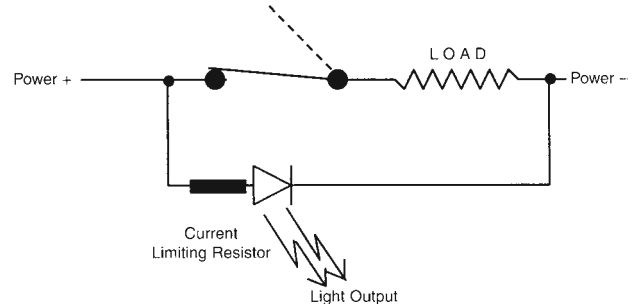
Figure 18. Wiring Diagram 3
