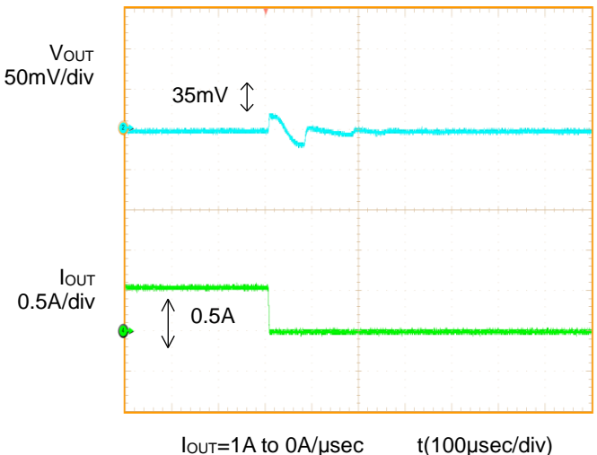
Figure 6. Transient Response (0.5A to 0A) C_{OUT}=22\mu F , C_{FB}=1000pF
