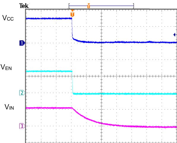
Figure 14. Waveform at Output OFF
