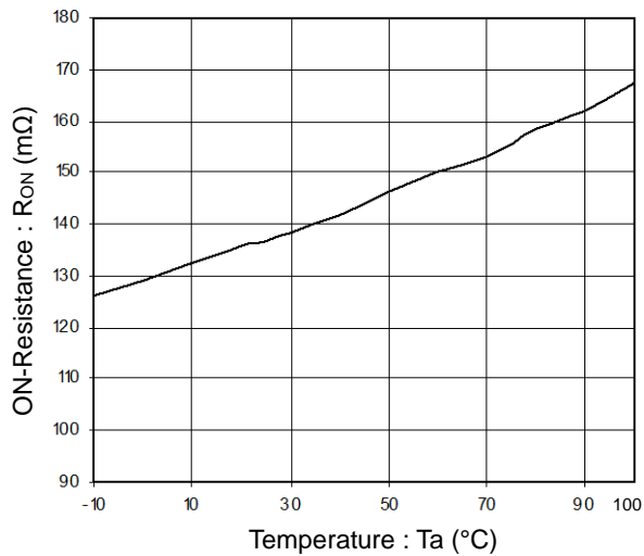
Figure 29. ON-Resistance vs Temperature ( V_{CC}=5V/V_{OUT}=1.2V )
