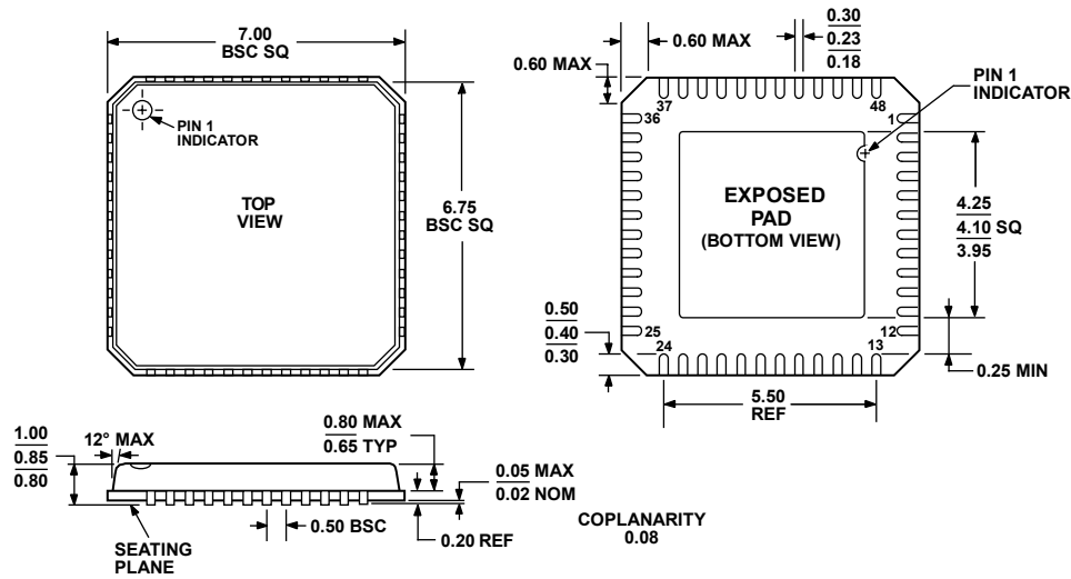
COMPLIANT TO JEDEC STANDARDS MO-220-VKDD-2 Figure 79. 48-Lead Lead Frame Chip Scale Package [LFCSP_VQ] 7 mm × 7 mm Body, Very Thin Quad (CP-48-3) Dimensions shown in millimeters
