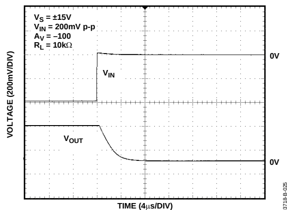
Figure 23. Positive Overdrive Recovery
