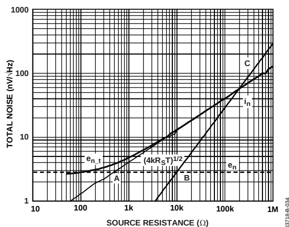
Figure 32. Noise vs. Source Resistance
