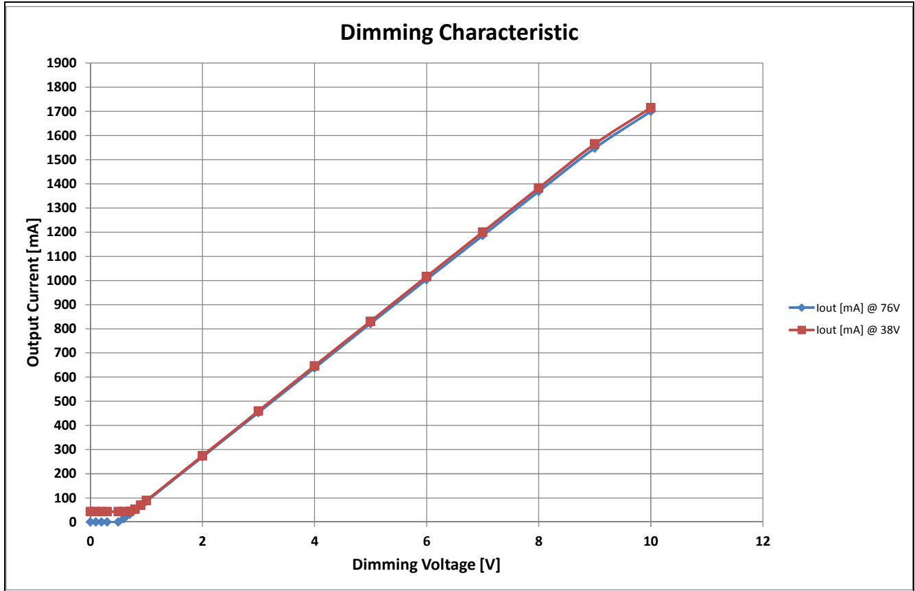
Output Current I OUT versus 0 – 10 V Dimming Voltage
